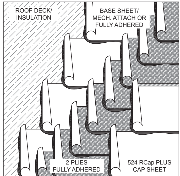
Four-ply, hot mopped, built-up roofing system with fiberglass base/ply sheets, and a highly-reflective, factory coated cap sheet installed over an approved roof deck.
